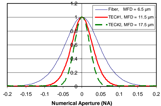
Fig. 2 Far-field measurement results with the TEC method
